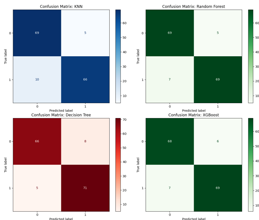
Fig. 8 Confusion matrix
