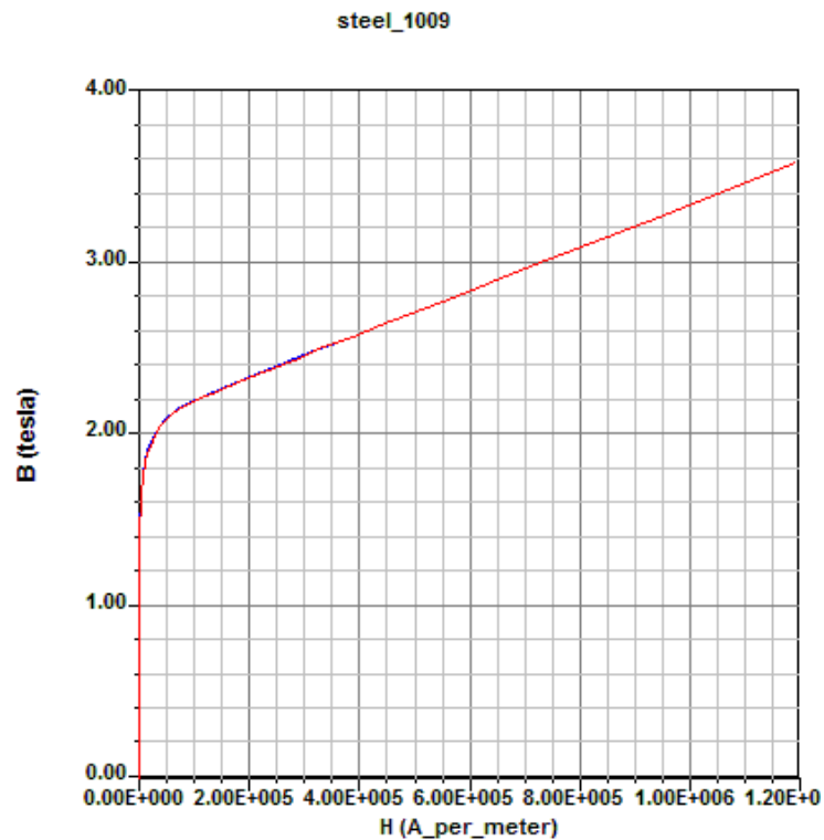
Fig.2 B-H curve of steel used for FEA
